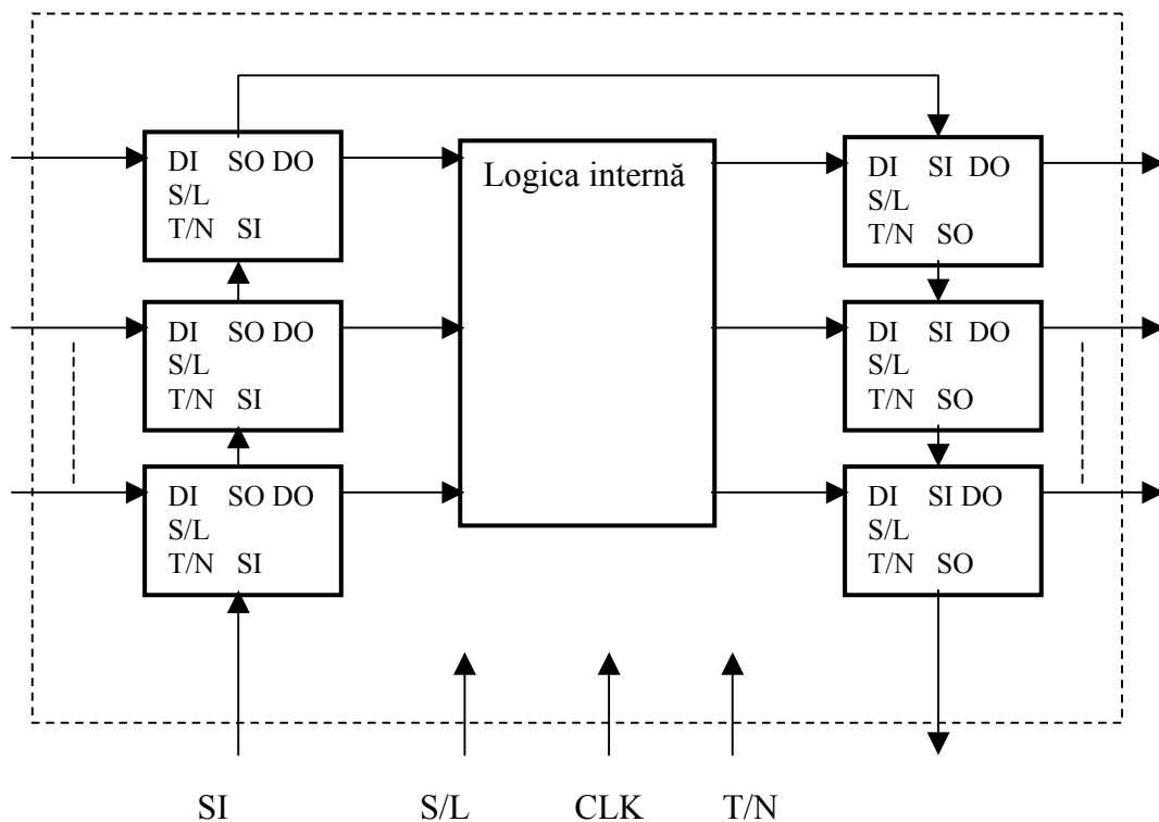
Figura 9.11: Structura BOUNDARY SCAN
