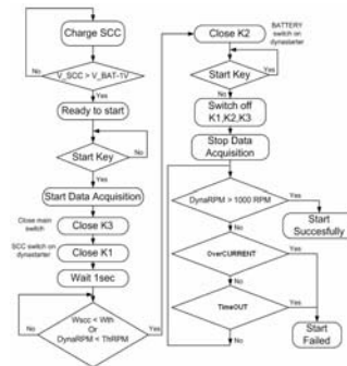
Fig. 3. Block diagram for starting the 6LDA28B ICE of the LDH1250HP locomotive
