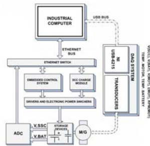
Fig. 1. General architecture of the prototype
