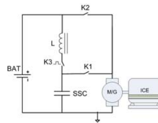
Fig. 2. Implemented starting system
